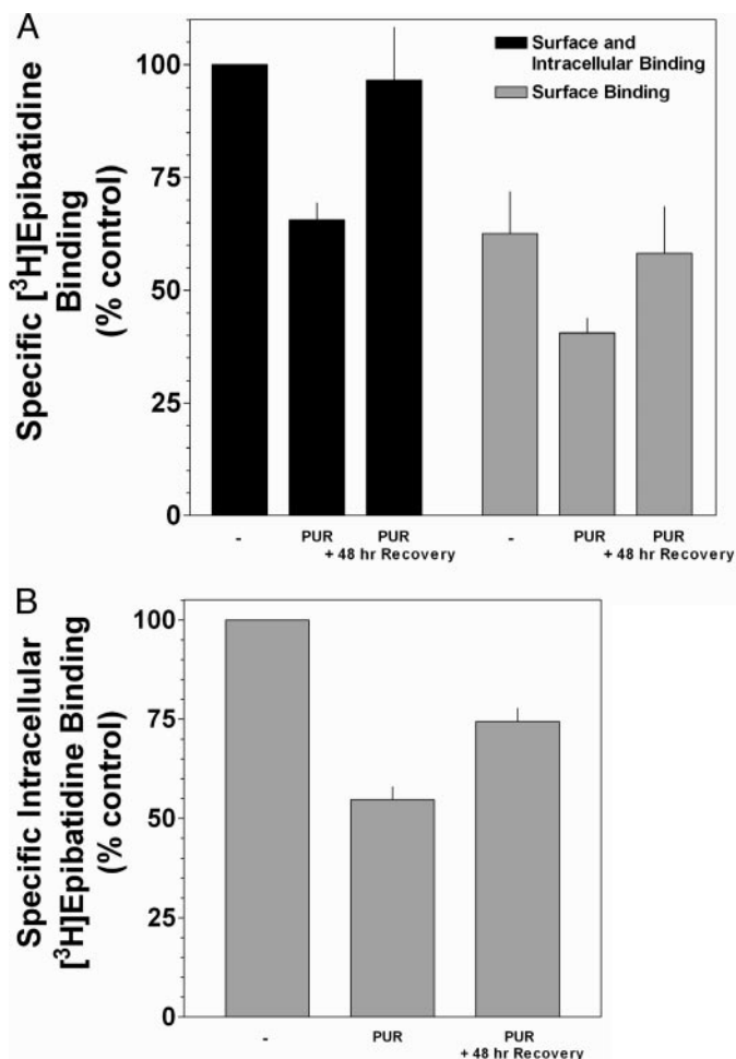
Fig. 5. A, effects of puromycin treatment on total and surface nAChRs. Cultured chromaffin cells were incubated either 1) with culture media for 24 h (–, control); 2) with culture media containing 10 μg/ml puromycin for 24 h (PUR); or 3) with culture media containing 10 μg/ml puromycin for 24 h, followed by a 48-h recovery period in media (PUR + 48 h Rec). After the treatment period, [ 3 H]epibatidine binding experiments (2 nM, ~80% receptor occupancy) were performed. To measure specific binding to both surface and intracellular nAChRs, the permeable, competitive ligand 300 μM nicotine was used (surface and intracellular binding). To measure specific binding to surface nAChRs, alone, the impermeable, competitive ligand 5 mM carbachol was used (surface binding). Data are represented as a percentage of control specific binding (1777 ± 185 cpm/culture). Values represent means ± S.E.M. (n = 4). B, effects of puromycin treatment on intracellular nAChRs. Cells were incubated either 1) with culture media for 24 h (–, control); 2) with culture media containing 10 μg/ml puromycin for 24 h (PUR); or 3) with culture media containing 10 μg/ml puromycin for 24 h, followed by a 48-h recovery period in media (PUR + 48 h Rec). To investigate the effects of puromycin treatment on intracellular binding, binding to surface nAChRs was eliminated by alkylation, as described under Materials and Methods . After puromycin treatment and alkylation, [ 3 H]epibatidine binding experiments (2 nM, ~80% receptor occupancy) were performed. Specific binding was measured using the permeable, competitive ligand 300 μM nicotine. Data are represented as a percentage of control specific binding (1463 ± 157 cpm/culture). Values represent means ± S.E.M. (n = 4).
