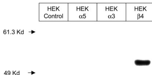
Fig. 6. Western Blot of transfected HEK cell extracts. Extracts (20 μg) from HEK control, HEK α5-transfected, HEK α3-transfected, or HEK β4-transfected cells were separated by 10% polyacrylamide gel electrophoresis and analyzed by Western blotting, as described under Materials and Methods . The blot was probed with a 1:1000 dilution of the anti-β4 nAChR polyclonal antibody PC 218, at 4°C overnight. After hybridization with anti-rabbit HRP-linked 2° antibody for 1 h, the blot was visualized by autoradiography using Amersham ECL.
