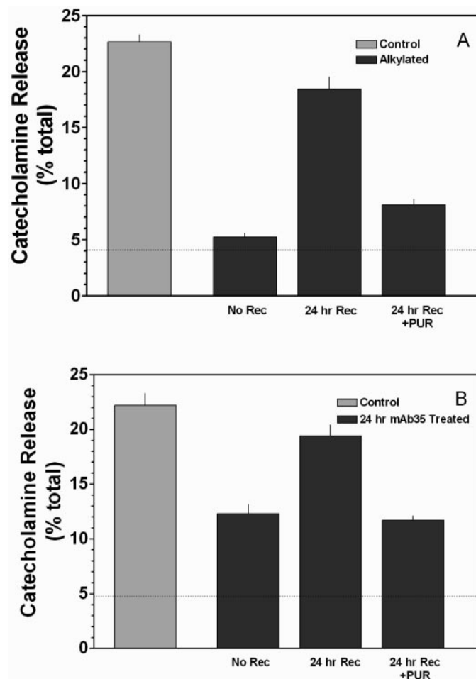
Fig. 3. Effects of puromycin on recovery of nAChRs after nAChR down-regulation. Cultured chromaffin cells were first loaded with [ ^3\text{H} ]NE, as described under Materials and Methods . A, effects of puromycin on recovery from alkylation-induced loss of functional surface nAChRs. Cells were either not treated (control) or alkylated using 100 \mu\text{M} bromoacetylcholine (alkylated). Some groups of alkylated cells were not allowed to recover and immediately stimulated (no Rec). Other groups were washed and allowed to recover by incubation for 24 h either in culture media (24 h Rec) or culture media containing 10 \mu\text{g}/\text{ml} puromycin (24 h Rec + PUR). B, effects of puromycin on recovery from mAb35 induced nAChR down-regulation. Cultured adrenal chromaffin cells were either not treated (control) or treated with 10 nM mAb35 for 24 h (24 h mAb35 treated). Some groups of mAb35-treated cells were not allowed to recover and stimulated immediately (no Rec). Other groups were washed and allowed to recover by incubation for 24 h either in culture media (24 h Rec) or culture media containing 10 \mu\text{g}/\text{ml} puromycin (24 h Rec + PUR). After all of these treatments, cells were washed (5 min) and then stimulated with 10 \mu\text{M} nicotine. Data are expressed as a percentage of total cellular [ ^3\text{H} ]NE content released during the 5-min stimulation period. Values are means \pm S.E.M. ( n = 4-6 ). Dashed line represents basal, nonstimulated, catecholamine release.
