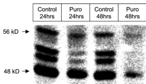
Fig. 7. Effects of puromycin treatment on nAChR \beta 4 protein levels. Cultured chromaffin cells were either not treated (control 24 h, control 48 h) or treated for 24 (puro 24 h) or 48 (puro 48 h) h in the presence of 10 \mu g/ml puromycin. After treatment, cells were washed once and extracted by scraping in extraction buffer. Samples were then analyzed via Western blot as described under Materials and Methods , probed with the anti- \beta 4 nAChR polyclonal antibody (described in Fig. 6), and visualized using ECL after incubation with an anti-rabbit HRP-conjugated antibody. Band size was determined by comparison with prestained protein standards. Data are shown as a representative blot. The four bands in the first lane starting with the top are 56, 52.2, 51, and 48 kDa.
