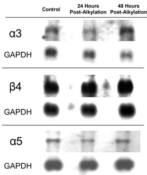
Fig. 2. Effects of alkylation-induced loss of functional surface nAChRs on nAChR subunit mRNA levels. Cells were alkylated and RNA was isolated immediately (control) and 24 and 48 h after alkylation. Northern blots were probed with bovine \beta 4 , \alpha 5 , and \alpha 3 cDNAs and then re-probed with GAPDH. The blots were exposed to film with an intensifying screen and then analyzed using a PhosphorImager to quantify the signal intensities in each lane. The nAChR subunit RNA signals were normalized to the GAPDH signals to measure relative changes in mRNA levels. The control signals were set at 100%. Slight changes in relative mRNA levels were seen which were not statistically significant ( \alpha 3 24 h, 98% and 48 h, 127%; \alpha 5 24 h, 86% and 48 h, 86%; and \beta 4 24 h, 96% and 48 h, 87%).
