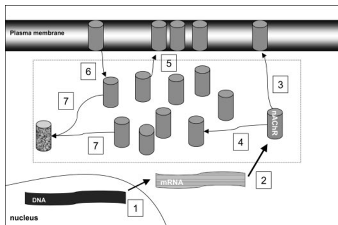
Fig. 8. Proposed model for surface expression of adrenal \alpha 3\beta 4^* nAChRs. Several steps may be involved with the expression of pentameric nAChRs (solid cylinders): 1, transcription; 2, translation; 3, trafficking of newly synthesized nAChRs to surface; 4, trafficking of newly synthesized nAChRs to intracellular pool (dotted box); 5, trafficking of nAChRs from intracellular pool to surface; 6, endocytosis of nAChRs from surface to intracellular pool; and 7, degradation of intracellular nAChRs (mottled cylinder). Additional description of the model is found in the text.
