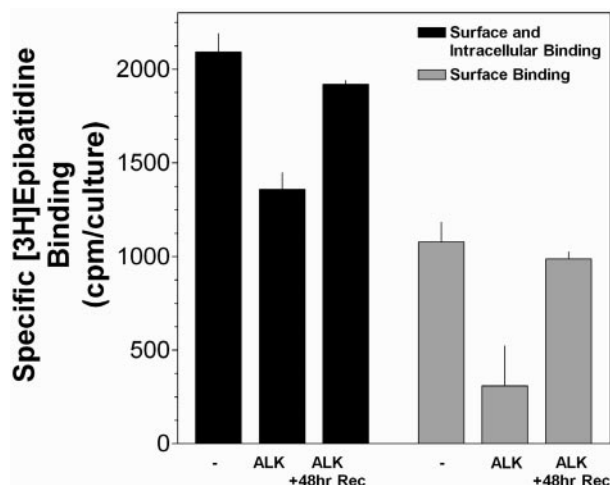
Fig. 1. Effects of alkylation and recovery from alkylation on [ ^3\text{H} ]epibatidine binding to cultured adrenal chromaffin cells. [ ^3\text{H} ]Epibatidine binding experiments (2 nM, ~80% receptor occupancy) were performed on the cells using either the permeable, competitive ligand 300 \mu\text{M} nicotine (surface and intracellular binding) to measure specific binding of the radioligand to both surface and intracellular nAChRs, or the impermeable, competitive ligand 5 mM carbachol (surface binding) to measure specific binding of the radioligand to surface nAChRs. Some cells were alkylated (ALK) before the binding reaction. In addition, some cells were alkylated and then allowed to recover by incubating in culture media for an additional 48 h (ALK + 48 h Rec) before the binding reaction. Data are represented as means \pm S.E.M. ( n = 4 ).
