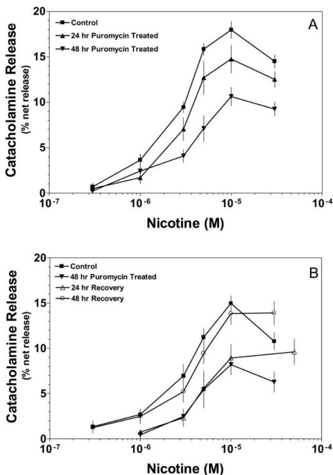
Fig. 4. A, time-dependent effects of puromycin on nicotine-stimulated adrenal secretion. Cultured adrenal chromaffin cells were first loaded with [ ^3\text{H} ]NE, as described under Materials and Methods . Cells were then incubated either 1) in culture media (control), 2) in 10 \mu\text{g/ml} puromycin for 24 h (24 h puromycin treated), or 3) in 10 \mu\text{g/ml} puromycin for 48 h (48 h puromycin treated). Cells were then washed and stimulated with the indicated concentrations of nicotine. Data are expressed as percentage of net stimulated release, i.e., total release minus basal release (mean \pm S.E.M.) for each concentration ( n = 4-6 ). B, time-dependent recovery of nicotine-stimulated secretion after puromycin treatment. Cells were first loaded with [ ^3\text{H} ]NE, as described under Materials and Methods . Cells were then incubated either 1) in culture media (control); 2) in 10 \mu\text{g/ml} puromycin for 48 h (48 h puromycin treated); 3) in 10 \mu\text{g/ml} puromycin for 48 h, followed by culture media for 24 h (24 h recovery); or 4) in 10 \mu\text{g/ml} puromycin for 48 h, followed by culture media for 48 h (48 h recovery). Cells were then washed and stimulated with the indicated concentrations of nicotine. Data are expressed as a percentage of stimulated release [i.e., total release minus basal release (mean \pm S.E.M.) for each concentration ( n = 3 )].
